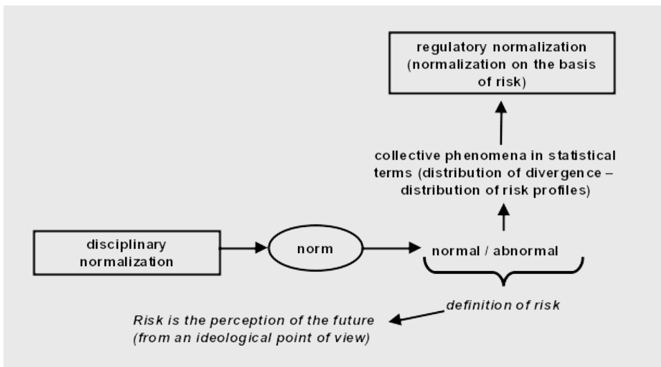
Figure 2. Normalization on the basis of risk
